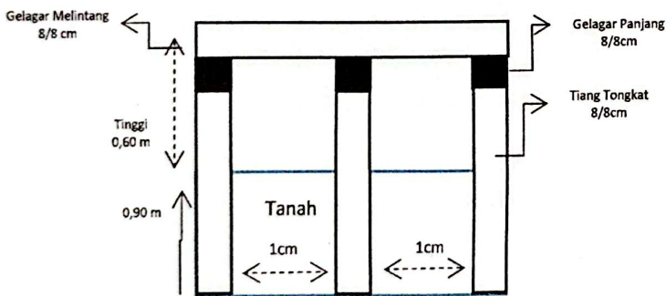
GAMBAR TAMPAK SAMPING
