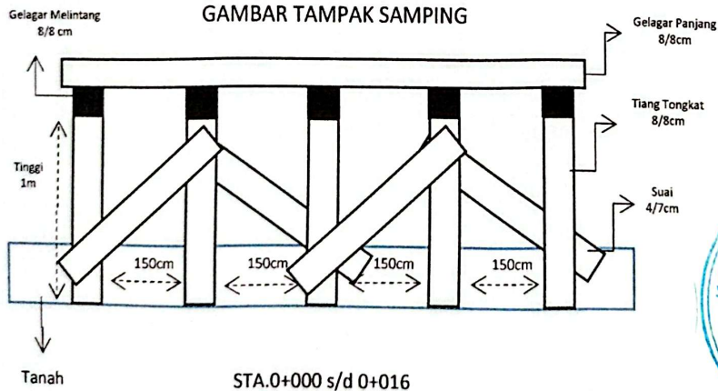
GAMBAR TAMPAK SAMPING
