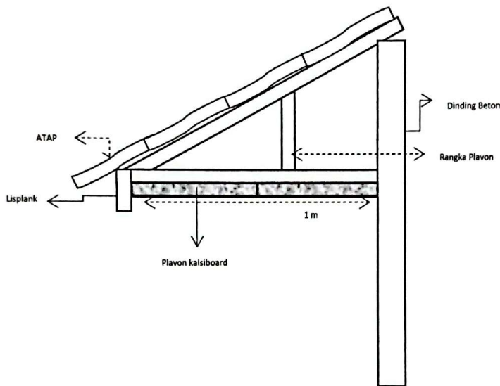
GAMBAR TAMPAK SAMPIING
