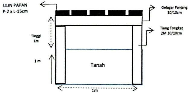
GAMBAR TAMPAK SAMPING
